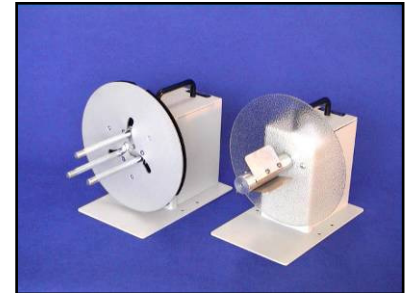
MC-11 (left): Rewind on any core from 1" to 4" diameter, or coreless.
